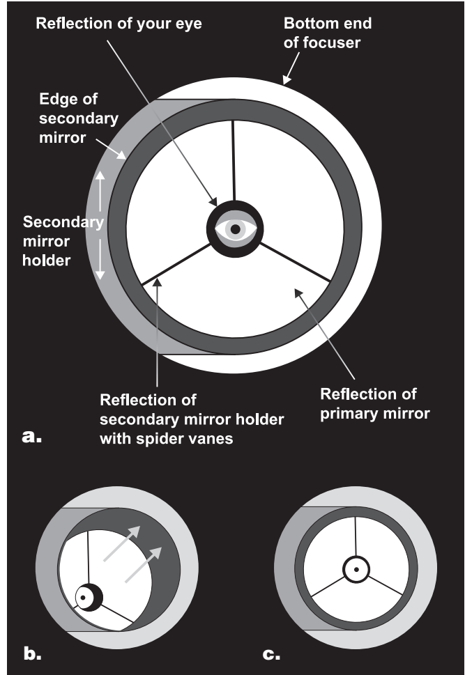
Figure 1. Collimating the optics. (a) When the mirrors are properly aligned, the view down the focuser drawtube should look like this; (b) With the collimation cap in place, if the optics are out of alignment, the view might look something like this; (c) After adjusting the secondary collimation setscrews, the reflection of the primary mirror should be centered in the secondary mirror as shown.
