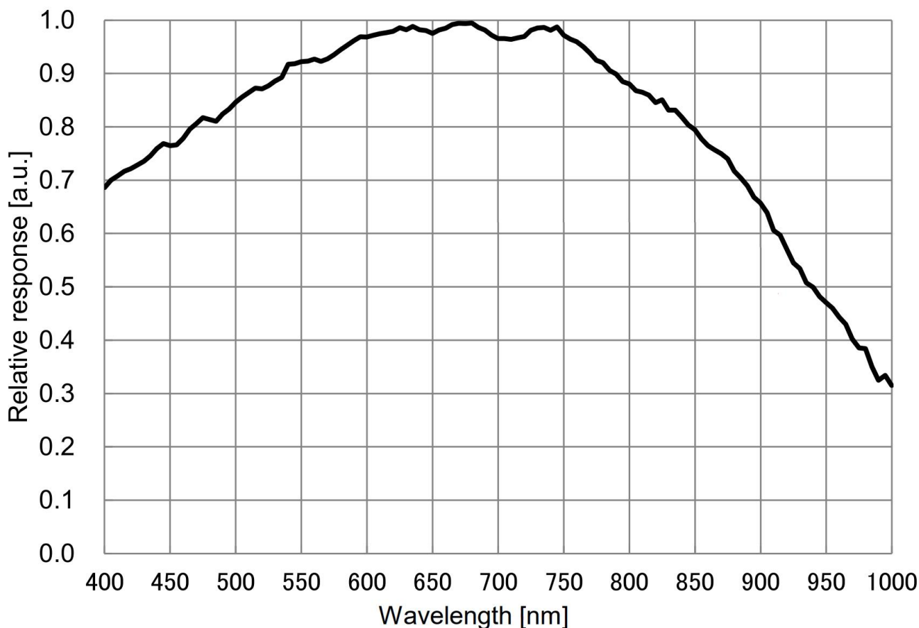
Figure 1 IMX676 Spectral Sensitivity Characteristic
