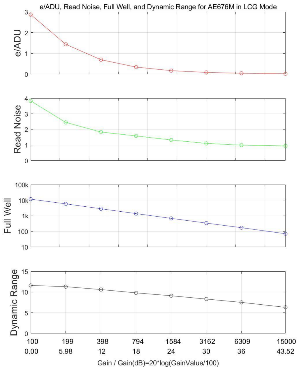
Figure 3 e/ADU, Read Noise, Full Well and Dynamic Range for AE676M
