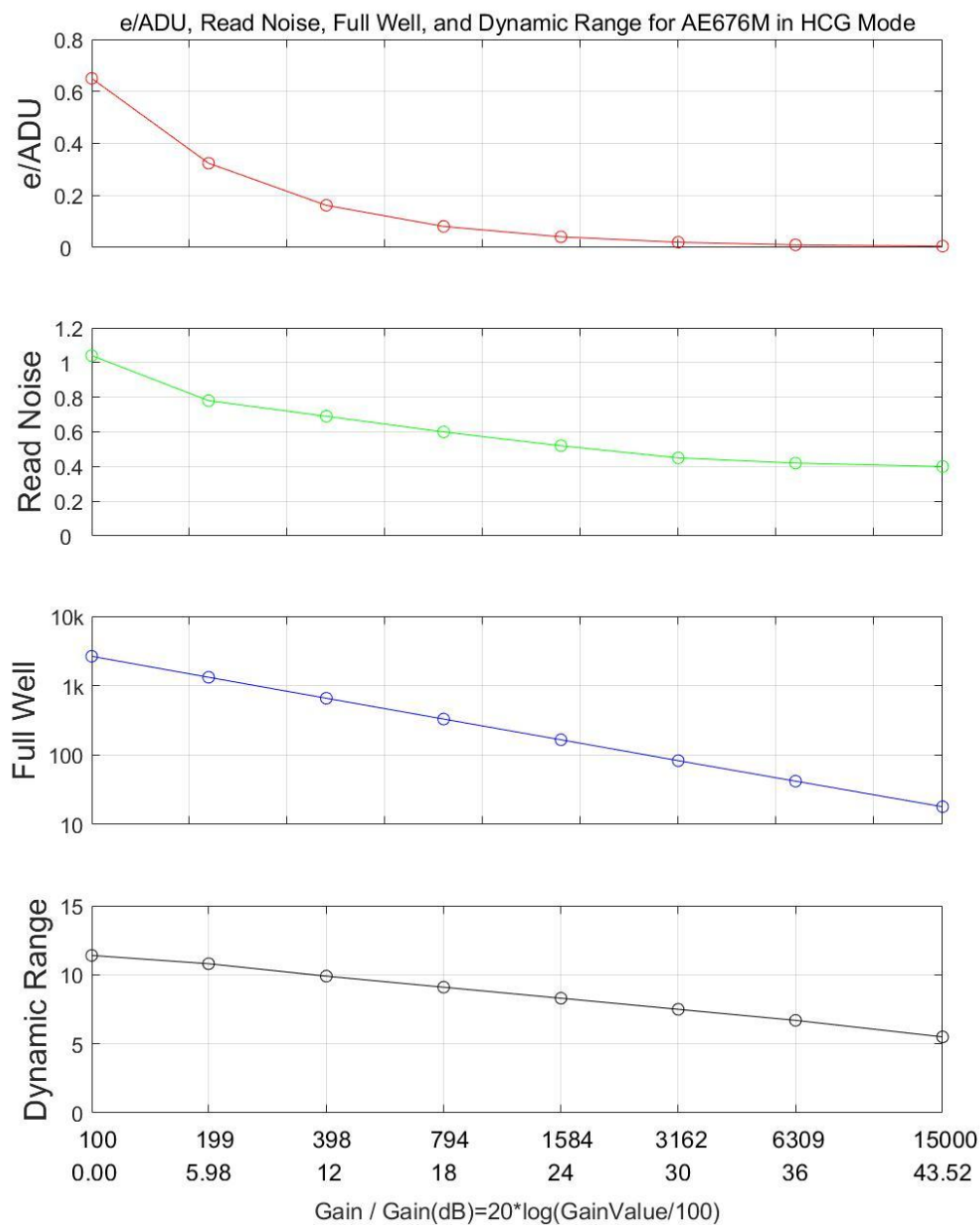
Figure 2 e/ADU, Read Noise, Full Well and Dynamic Range for AE676M
