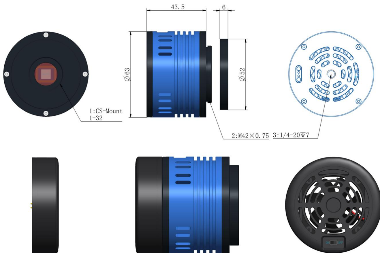
Figure 5 Dimension and Mount of AE676M
